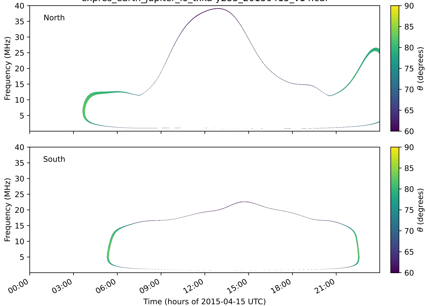
expres_earth_jupiter_io_txka-y235_20150415_v14.cdf
