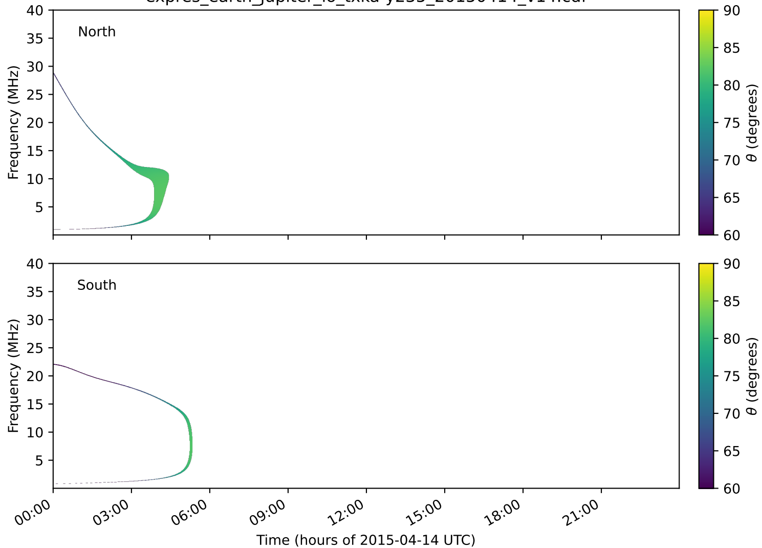
expres_earth_jupiter_io_txka-y235_20150414_v14.cdf
