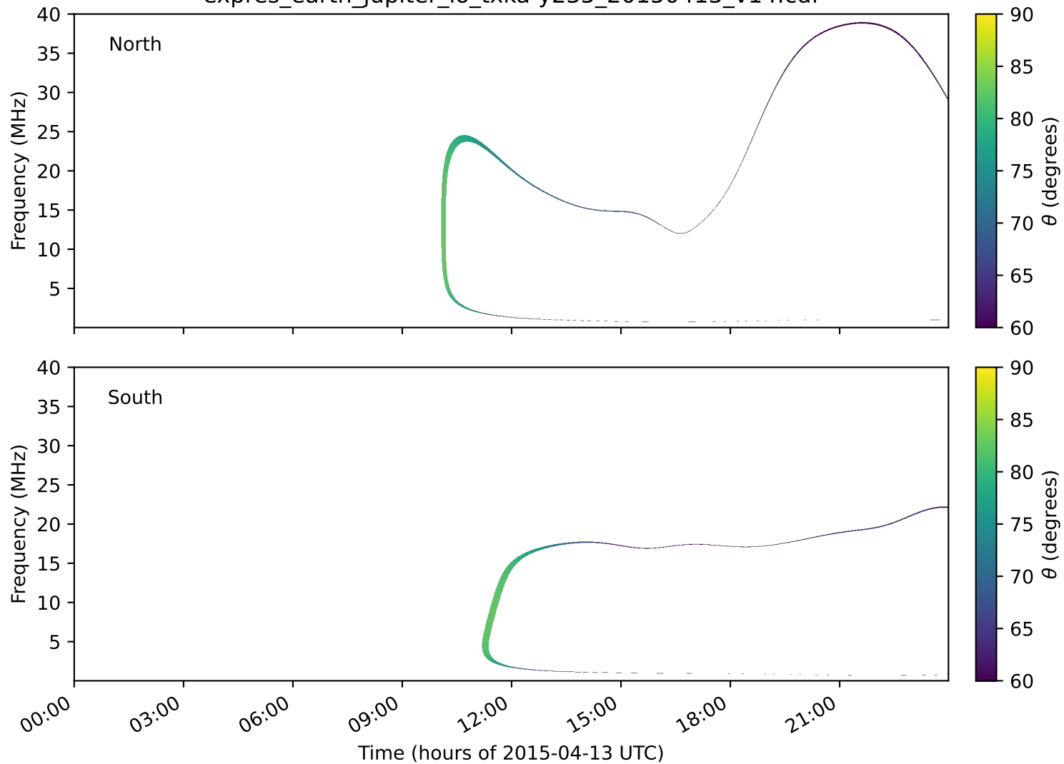
expres_earth_jupiter_io_txka-y235_20150413_v14.cdf
