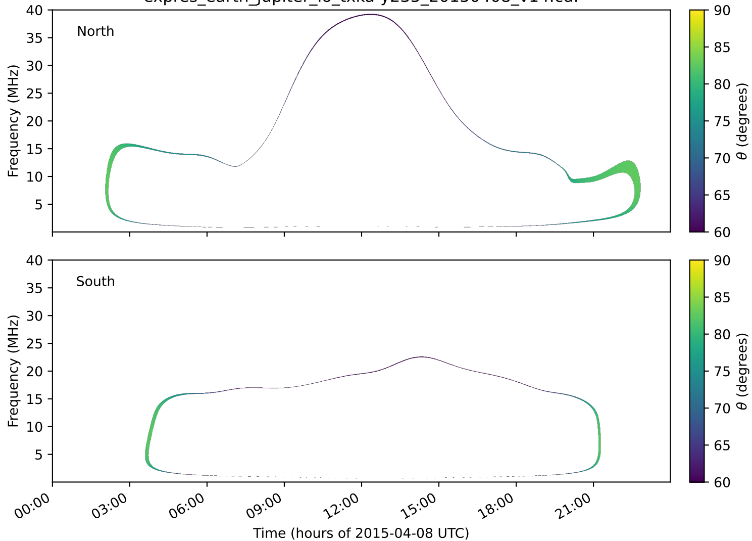
expres_earth_jupiter_io_txka-y235_20150408_v14.cdf
