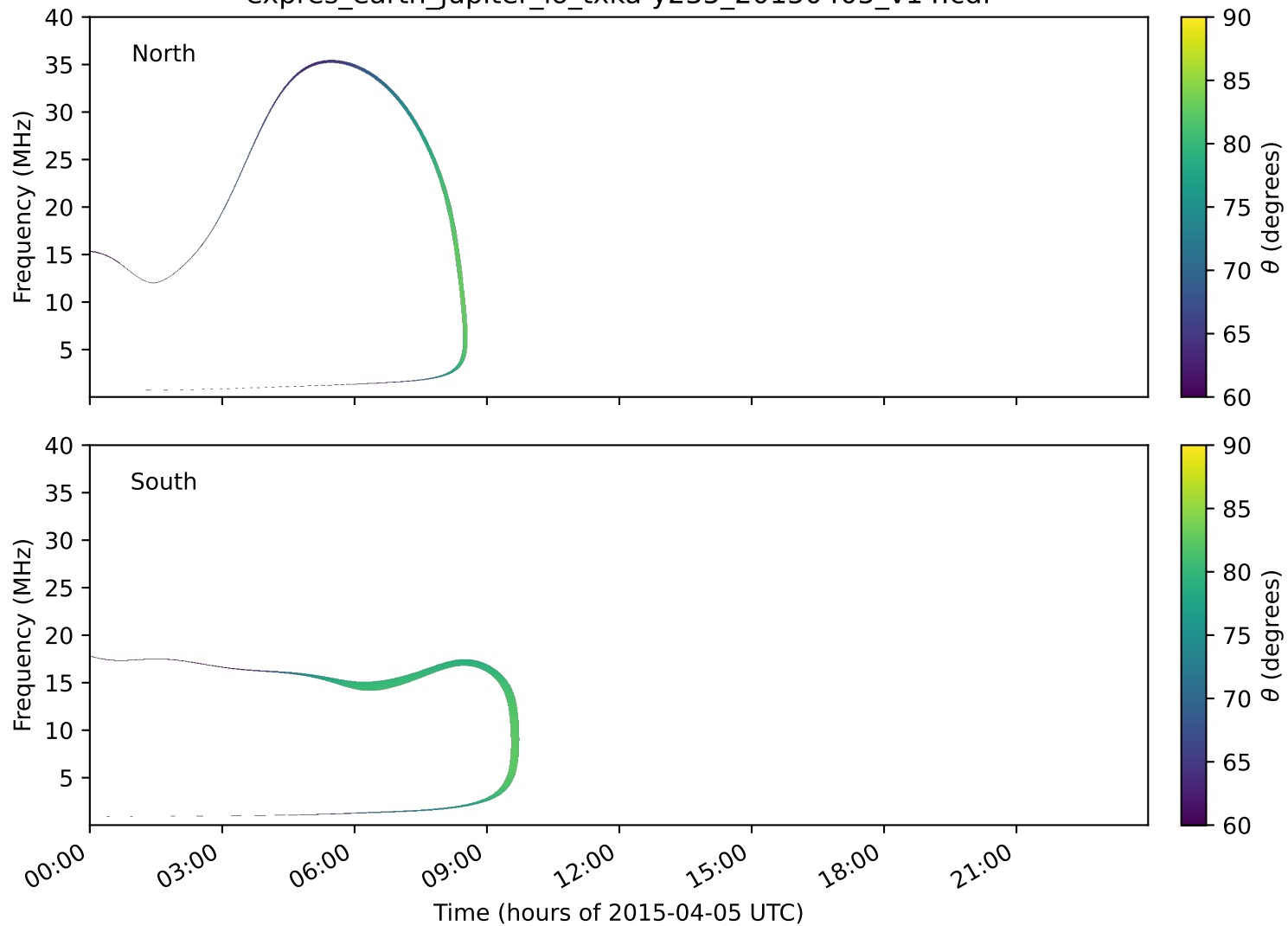
expres_earth_jupiter_io_txka-y235_20150405_v14.cdf
