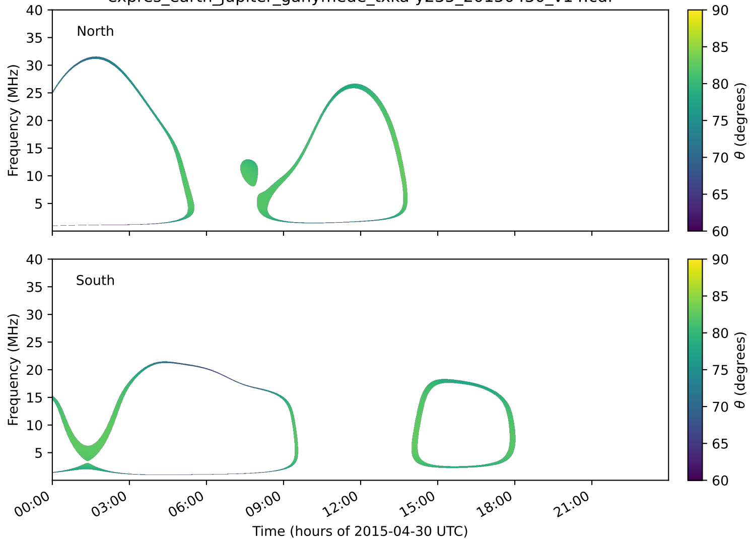
expres_earth_jupiter_ganymede_txka-y235_20150430_v14.cdf
