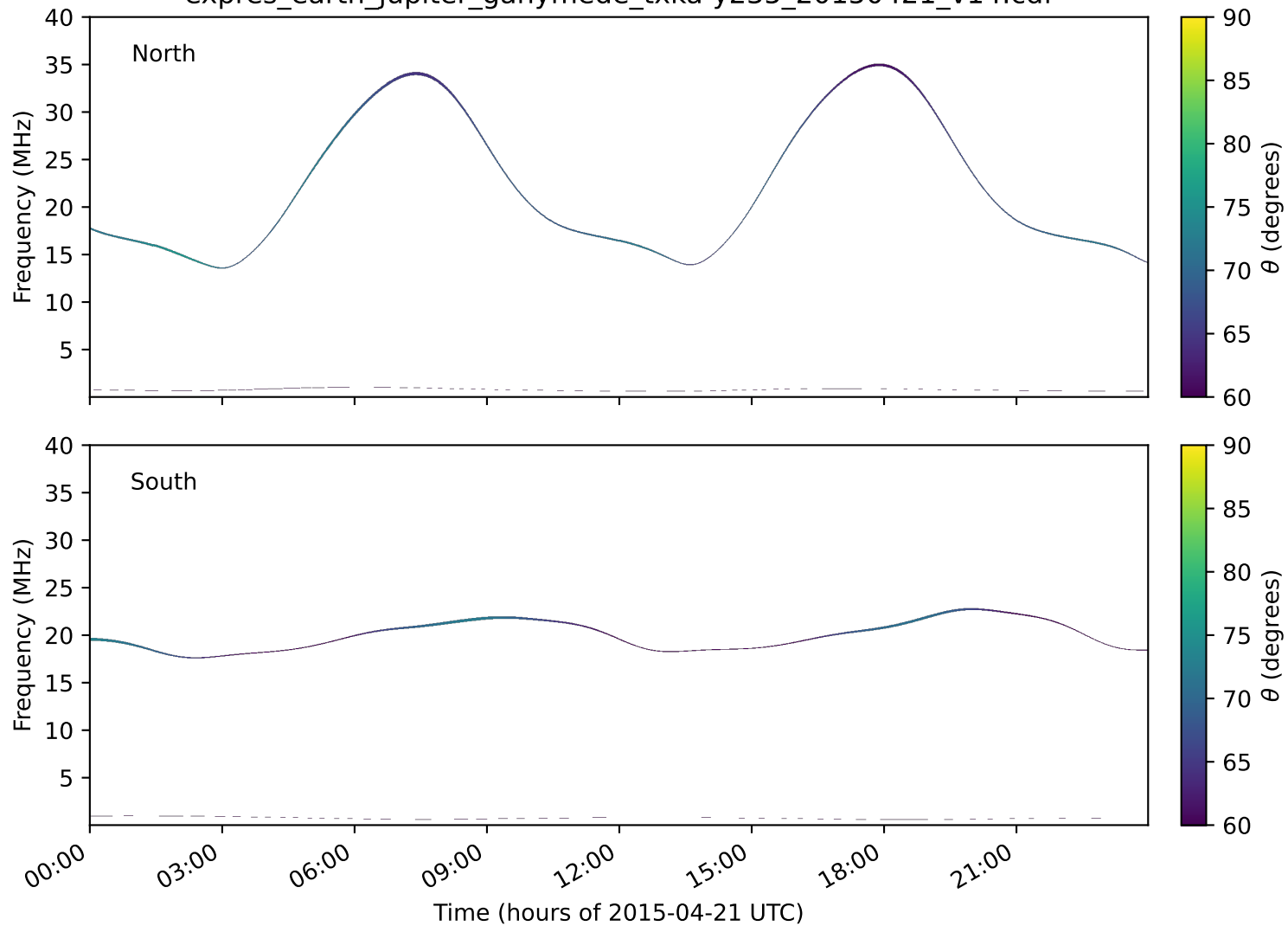
expres_earth_jupiter_ganymede_txka-y235_20150421_v14.cdf
