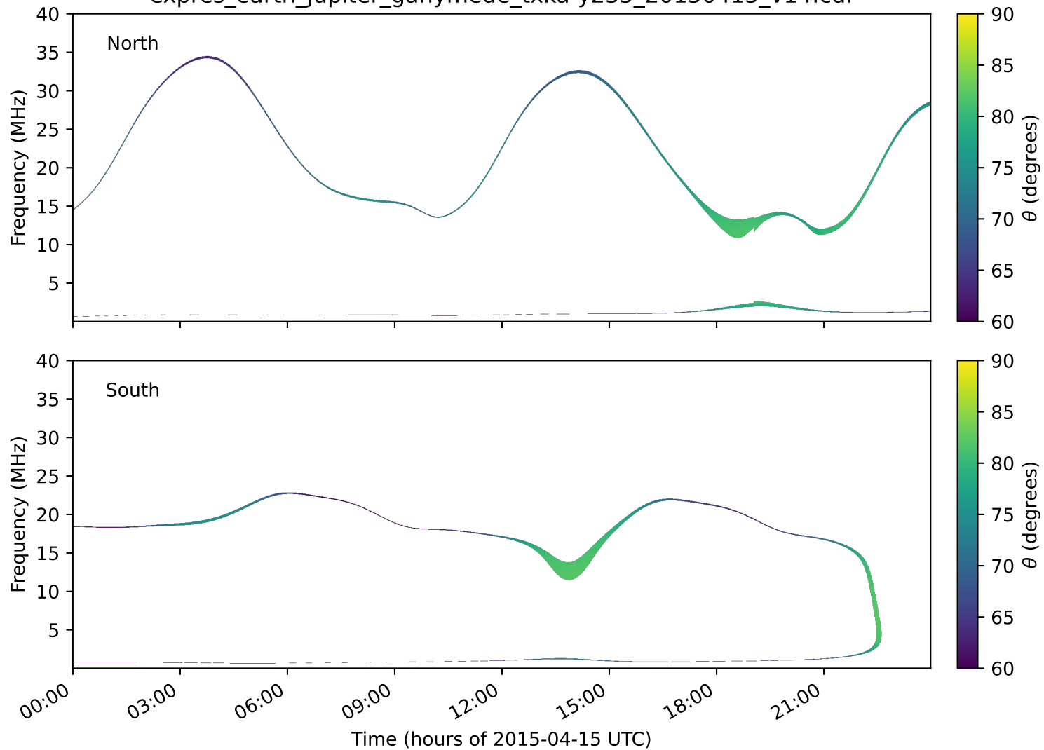
expres_earth_jupiter_ganymede_txka-y235_20150415_v14.cdf
