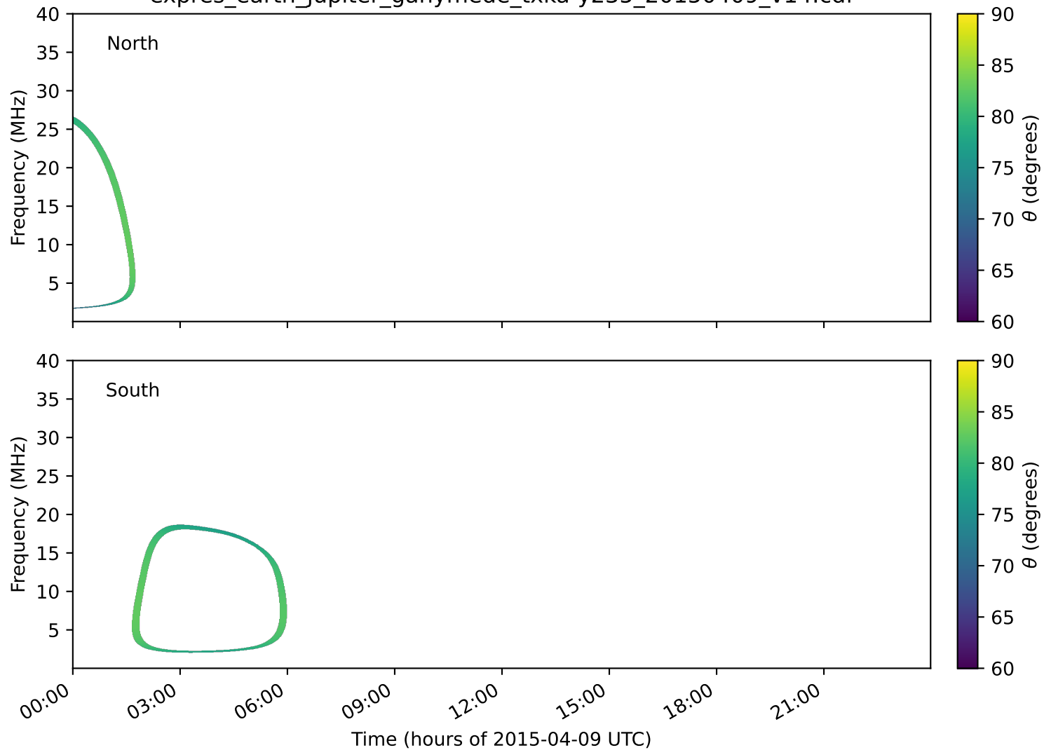
expres_earth_jupiter_ganymede_txka-y235_20150409_v14.cdf
