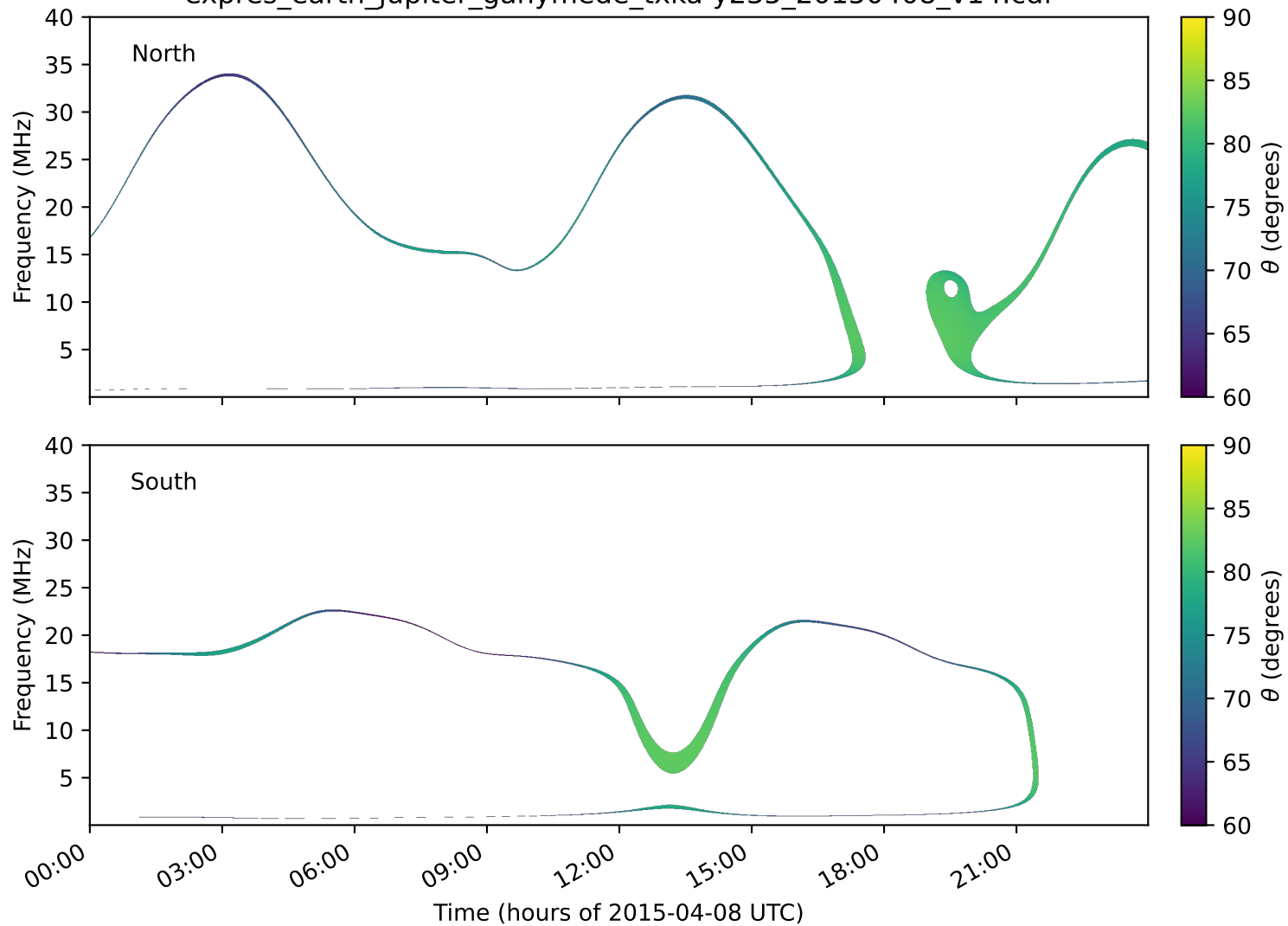
expres_earth_jupiter_ganymede_txka-y235_20150408_v14.cdf
