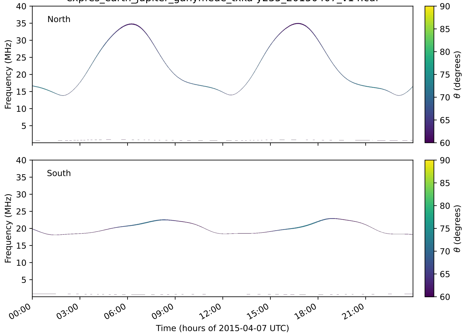
expres_earth_jupiter_ganymede_txka-y235_20150407_v14.cdf
