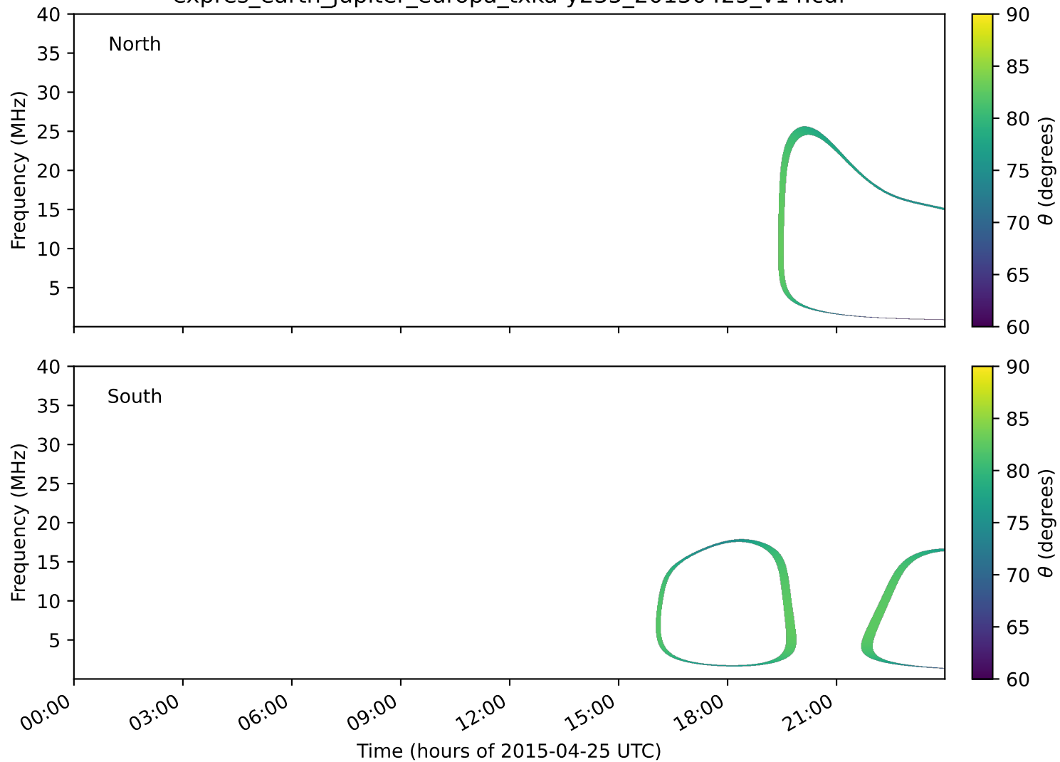
expres_earth_jupiter_europa_txka-y235_20150425_v14.cdf
