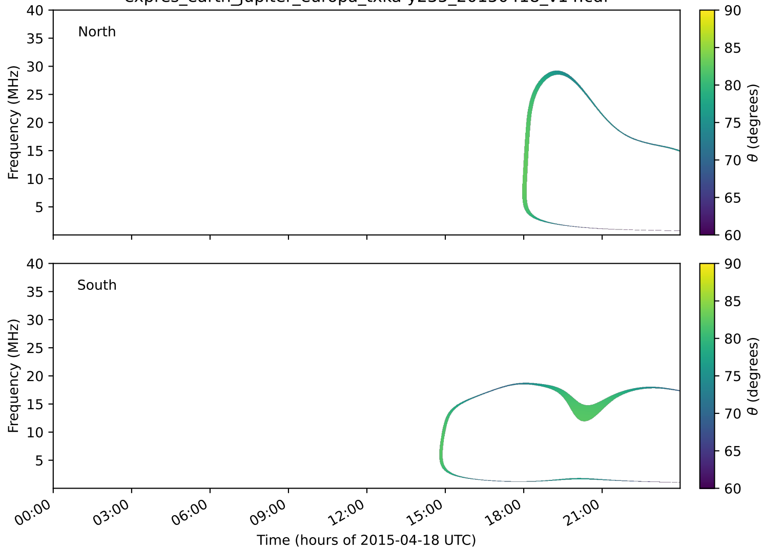
expres_earth_jupiter_europa_txka-y235_20150418_v14.cdf
