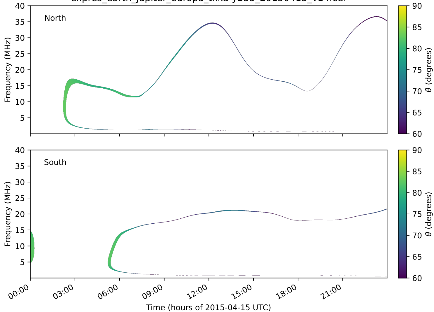
expres_earth_jupiter_europa_txka-y235_20150415_v14.cdf
