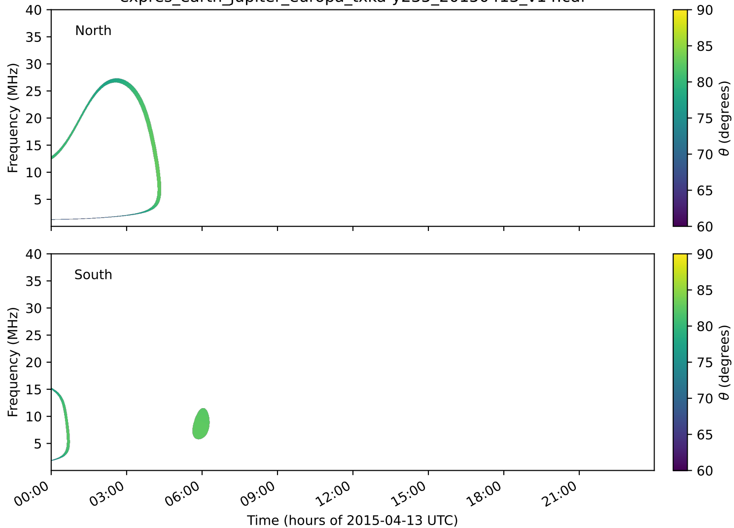
expres_earth_jupiter_europa_txka-y235_20150413_v14.cdf
