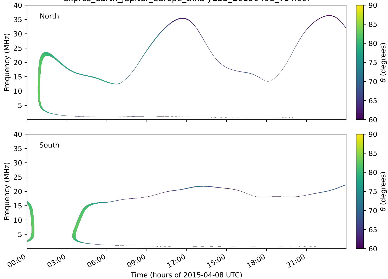
expres_earth_jupiter_europa_txka-y235_20150408_v14.cdf
