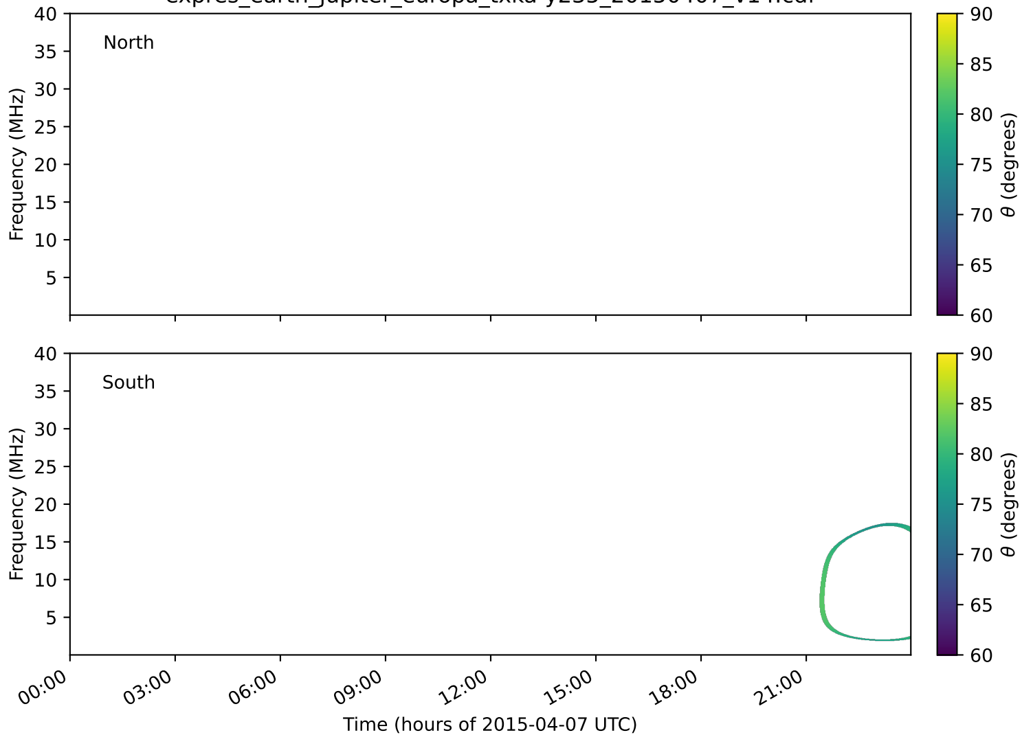
expres_earth_jupiter_europa_txka-y235_20150407_v14.cdf
