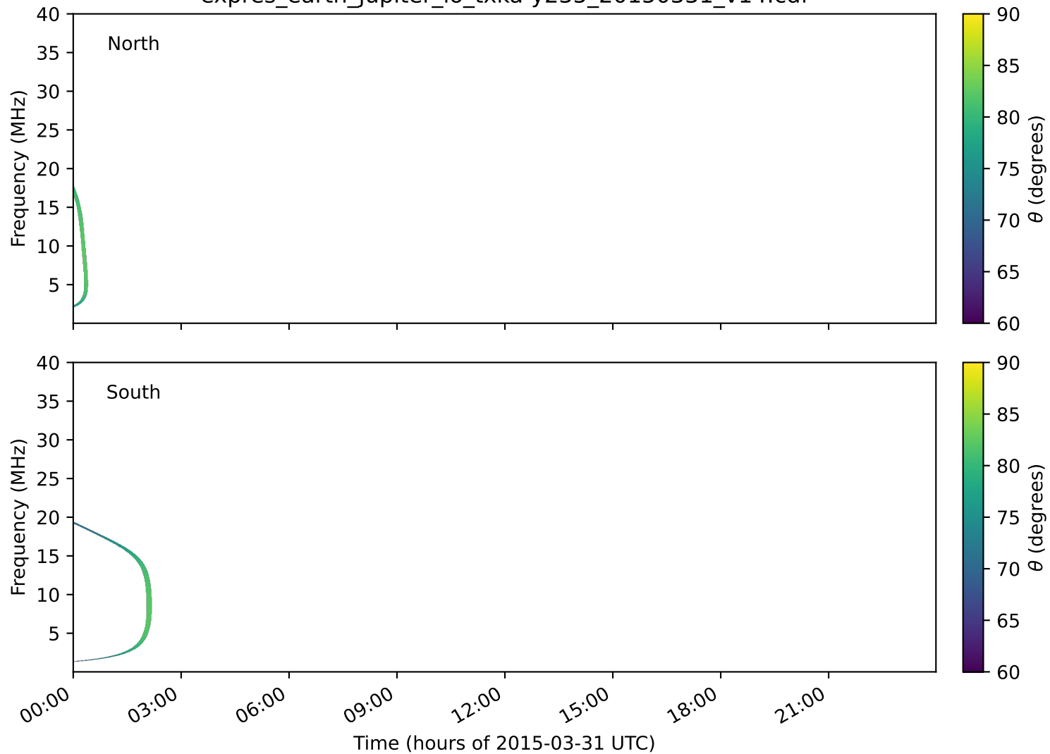
expres_earth_jupiter_io_txka-y235_20150331_v14.cdf
