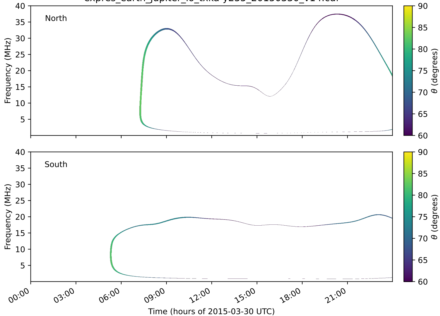
expres_earth_jupiter_io_txka-y235_20150330_v14.cdf
