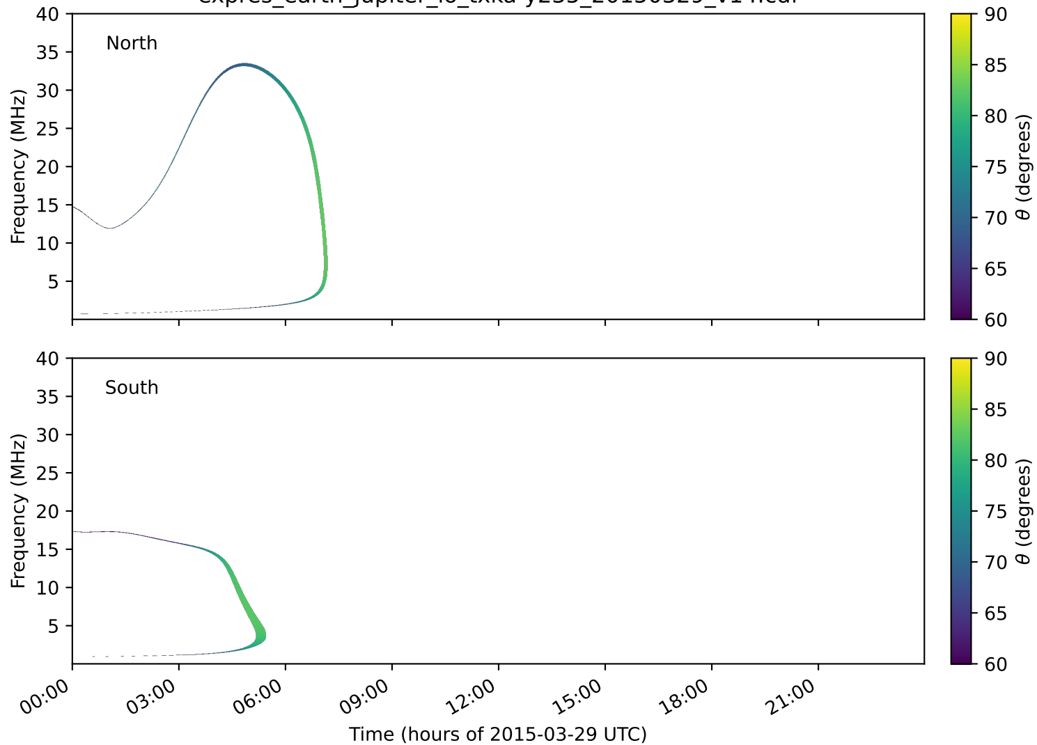
expres_earth_jupiter_io_txka-y235_20150329_v14.cdf
