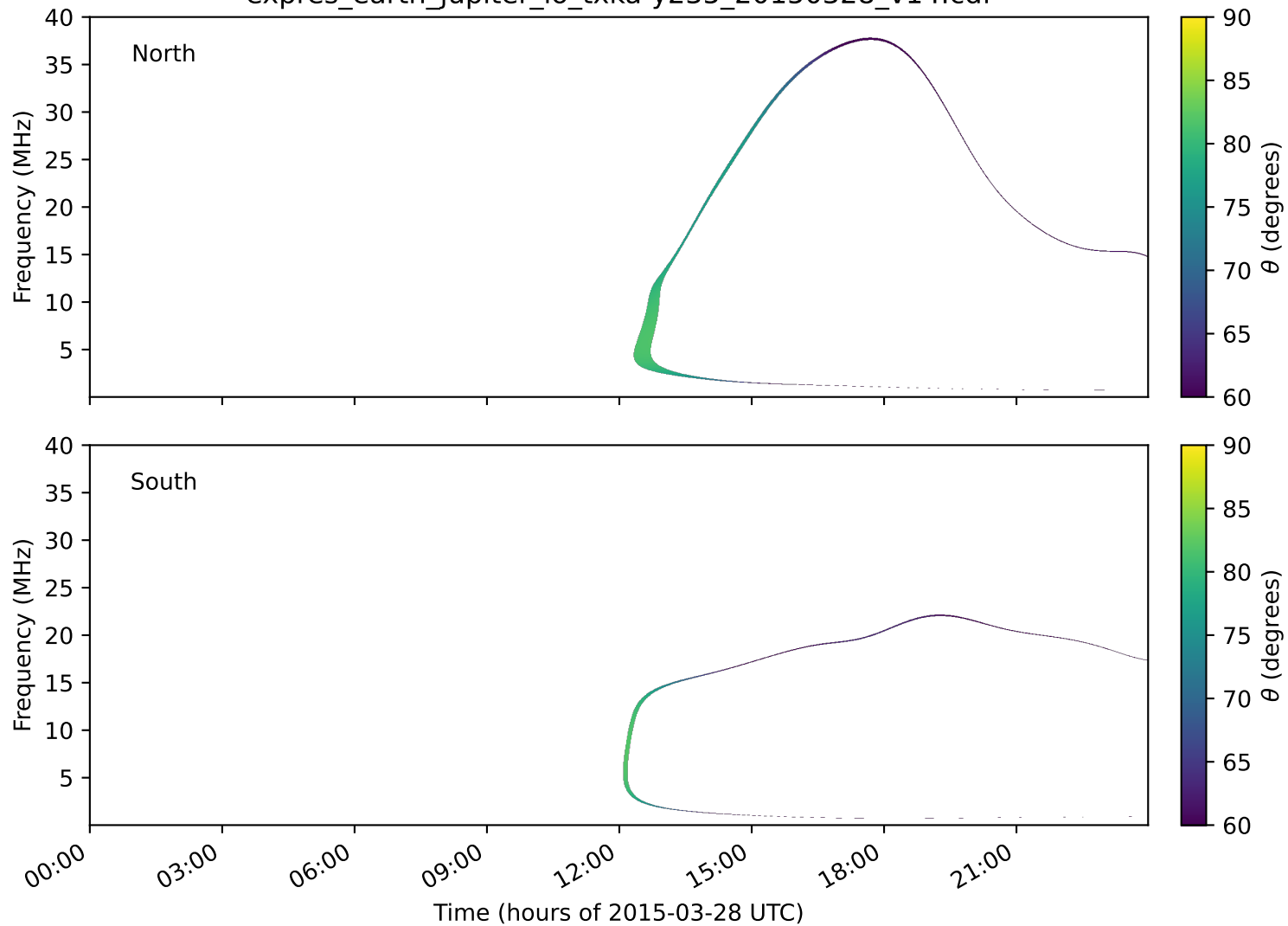
expres_earth_jupiter_io_txka-y235_20150328_v14.cdf
