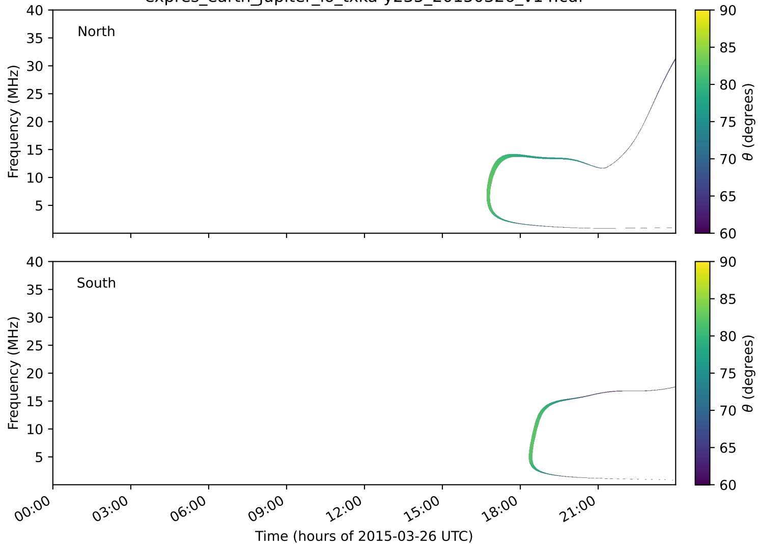
expres_earth_jupiter_io_txka-y235_20150326_v14.cdf
