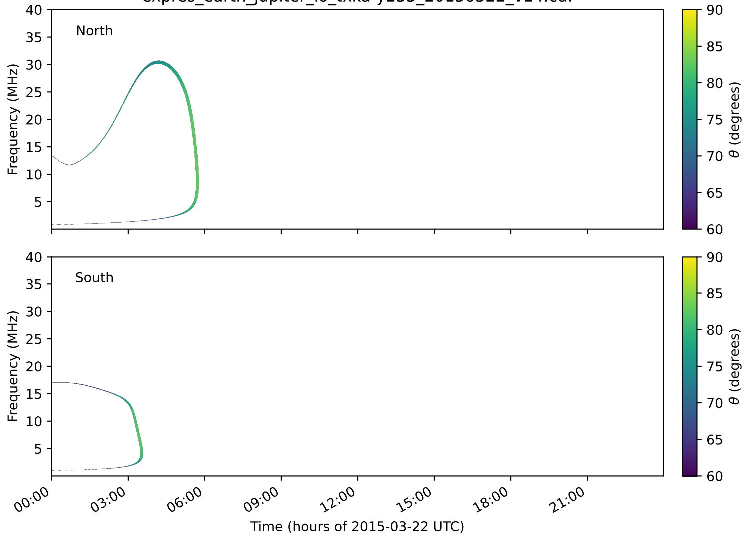
expres_earth_jupiter_io_txka-y235_20150322_v14.cdf
