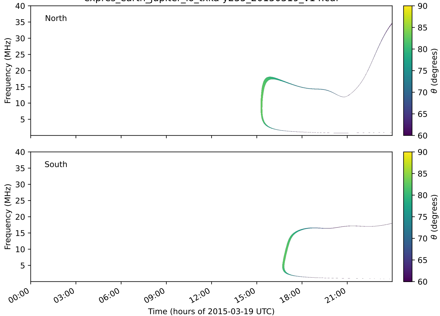
expres_earth_jupiter_io_txka-y235_20150319_v14.cdf
