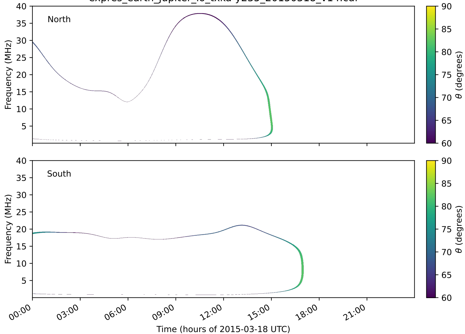
expres_earth_jupiter_io_txka-y235_20150318_v14.cdf
