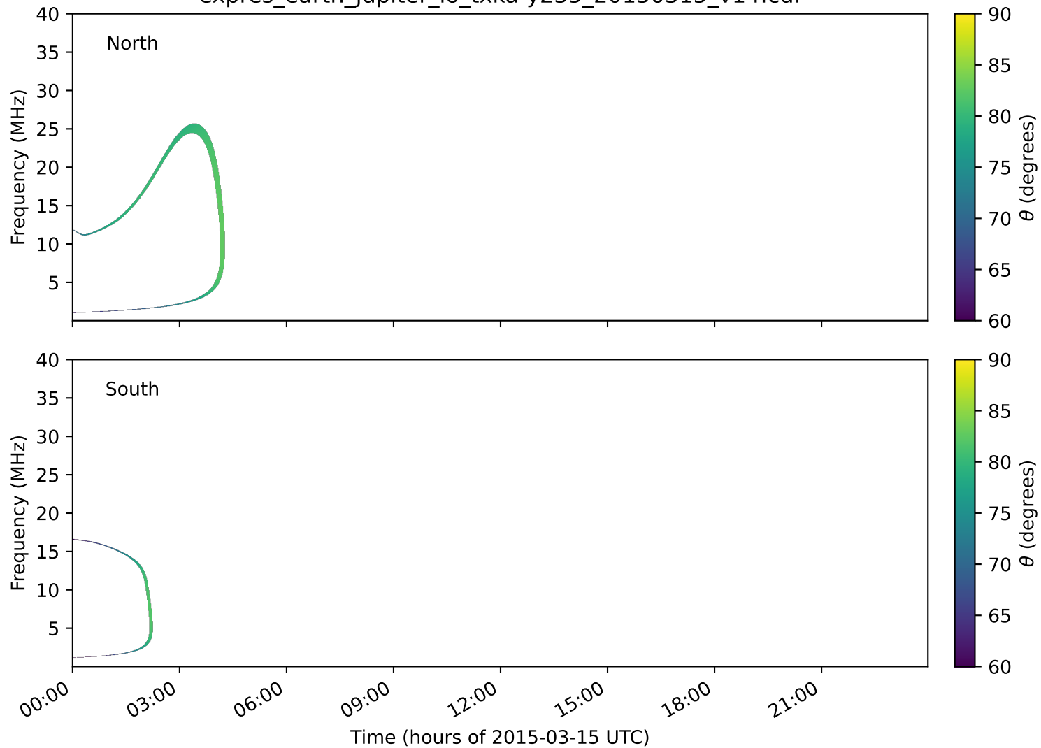
expres_earth_jupiter_io_txka-y235_20150315_v14.cdf
