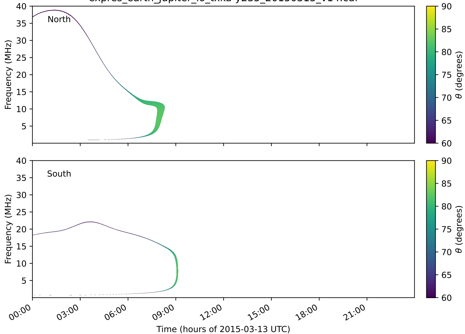
expres_earth_jupiter_io_txka-y235_20150313_v14.cdf
