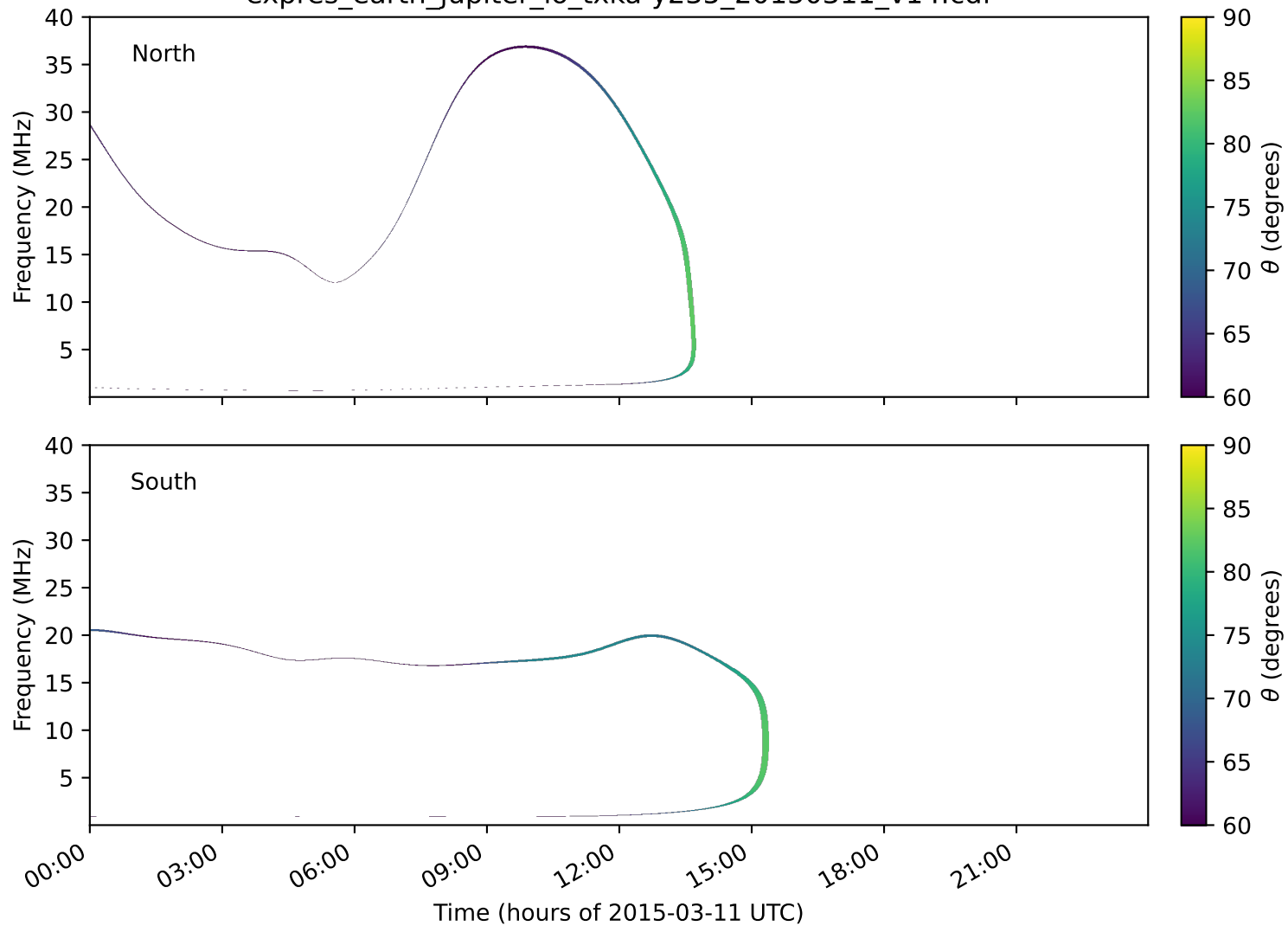
expres_earth_jupiter_io_txka-y235_20150311_v14.cdf
