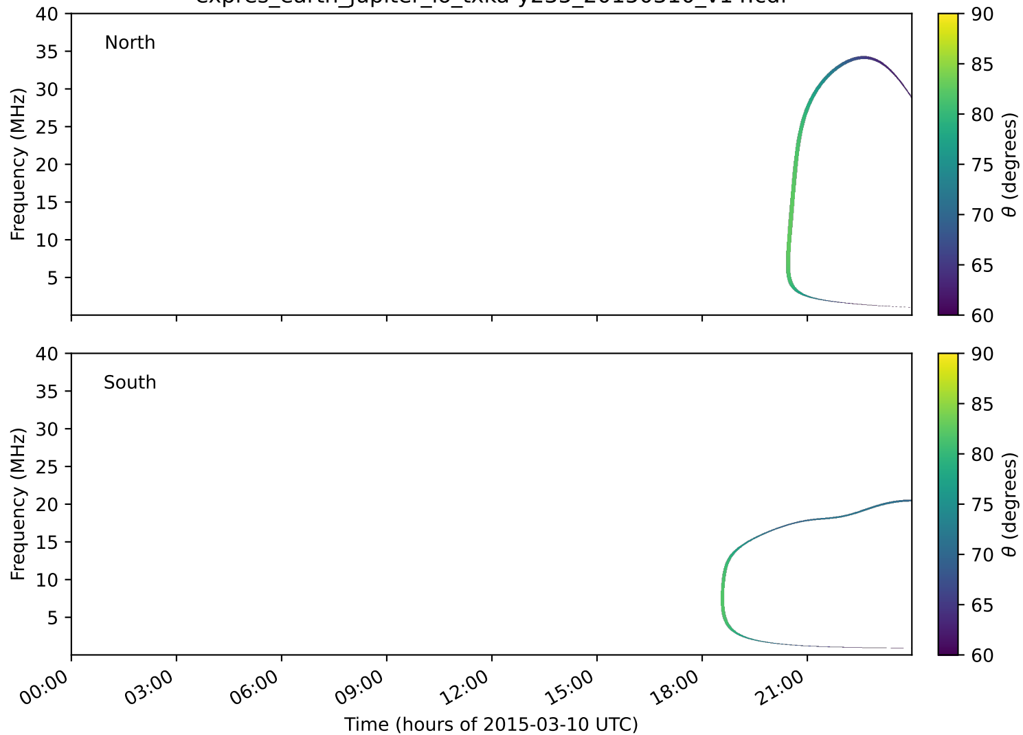
expres_earth_jupiter_io_txka-y235_20150310_v14.cdf
