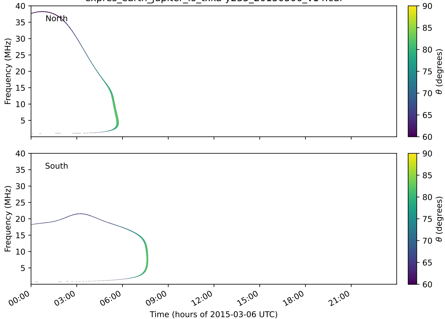
expres_earth_jupiter_io_txka-y235_20150306_v14.cdf
