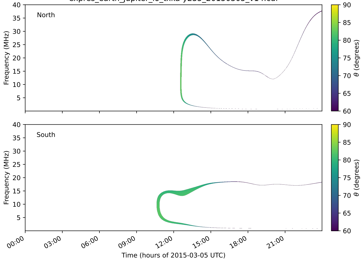
expres_earth_jupiter_io_txka-y235_20150305_v14.cdf
