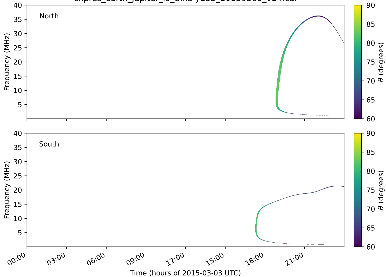
expres_earth_jupiter_io_txka-y235_20150303_v14.cdf
