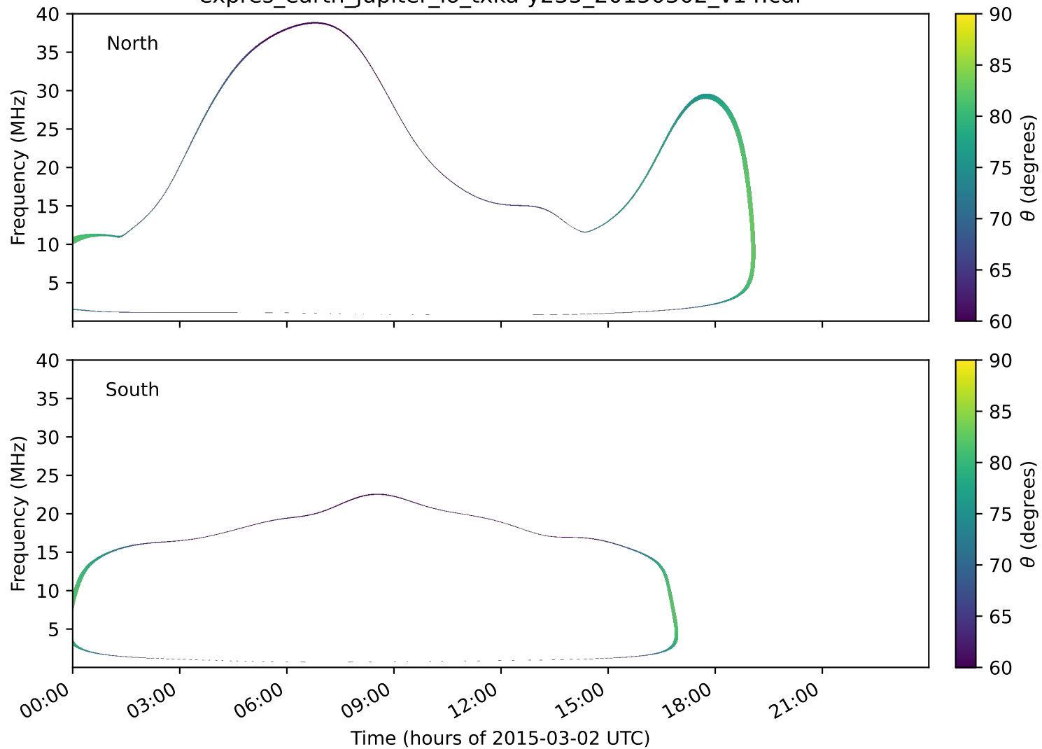
expres_earth_jupiter_io_txka-y235_20150302_v14.cdf
