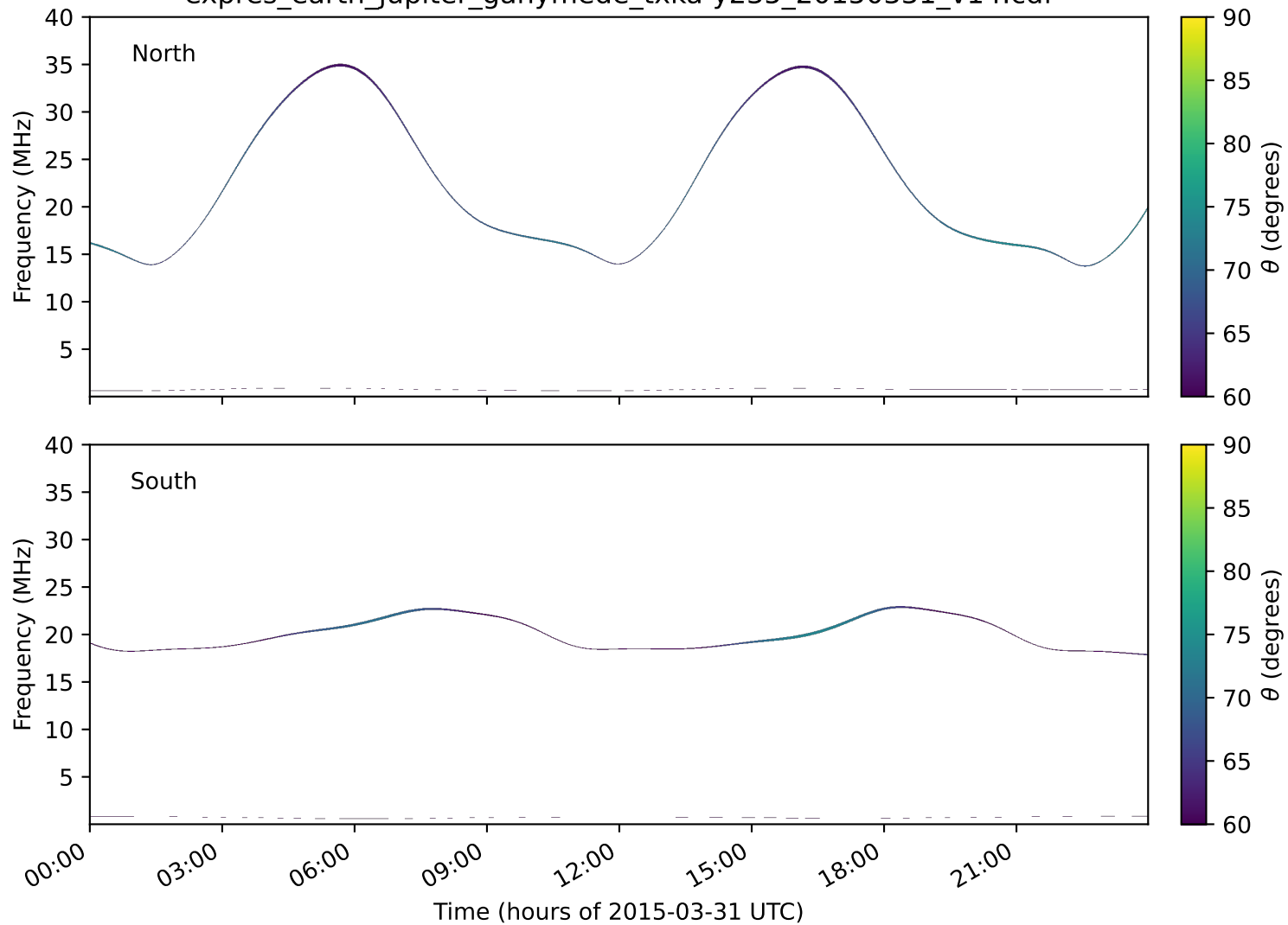
expres_earth_jupiter_ganymede_txka-y235_20150331_v14.cdf
