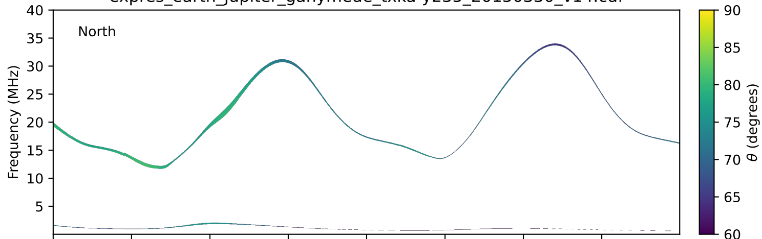
expres_earth_jupiter_ganymede_txka-y235_20150330_v14.cdf
