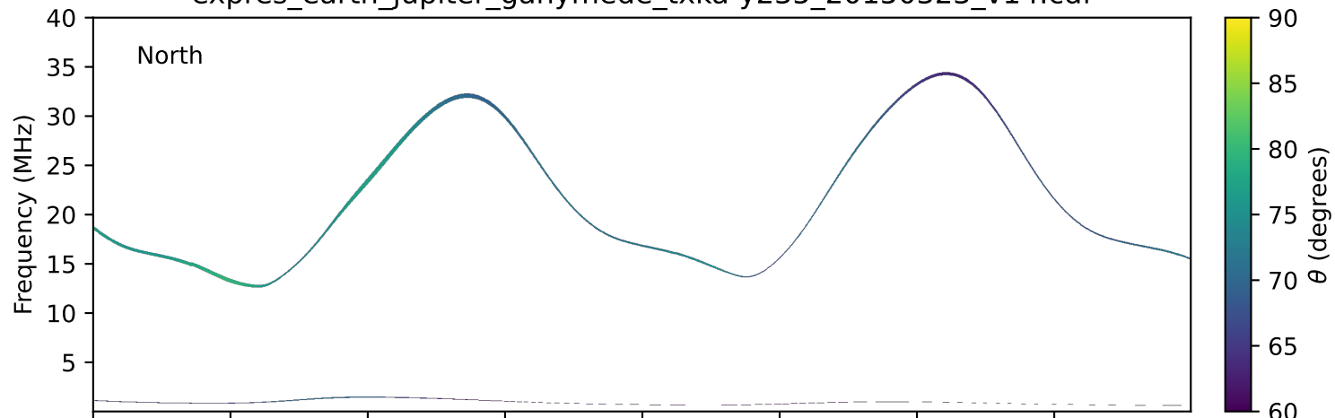
expres_earth_jupiter_ganymede_txka-y235_20150323_v14.cdf
