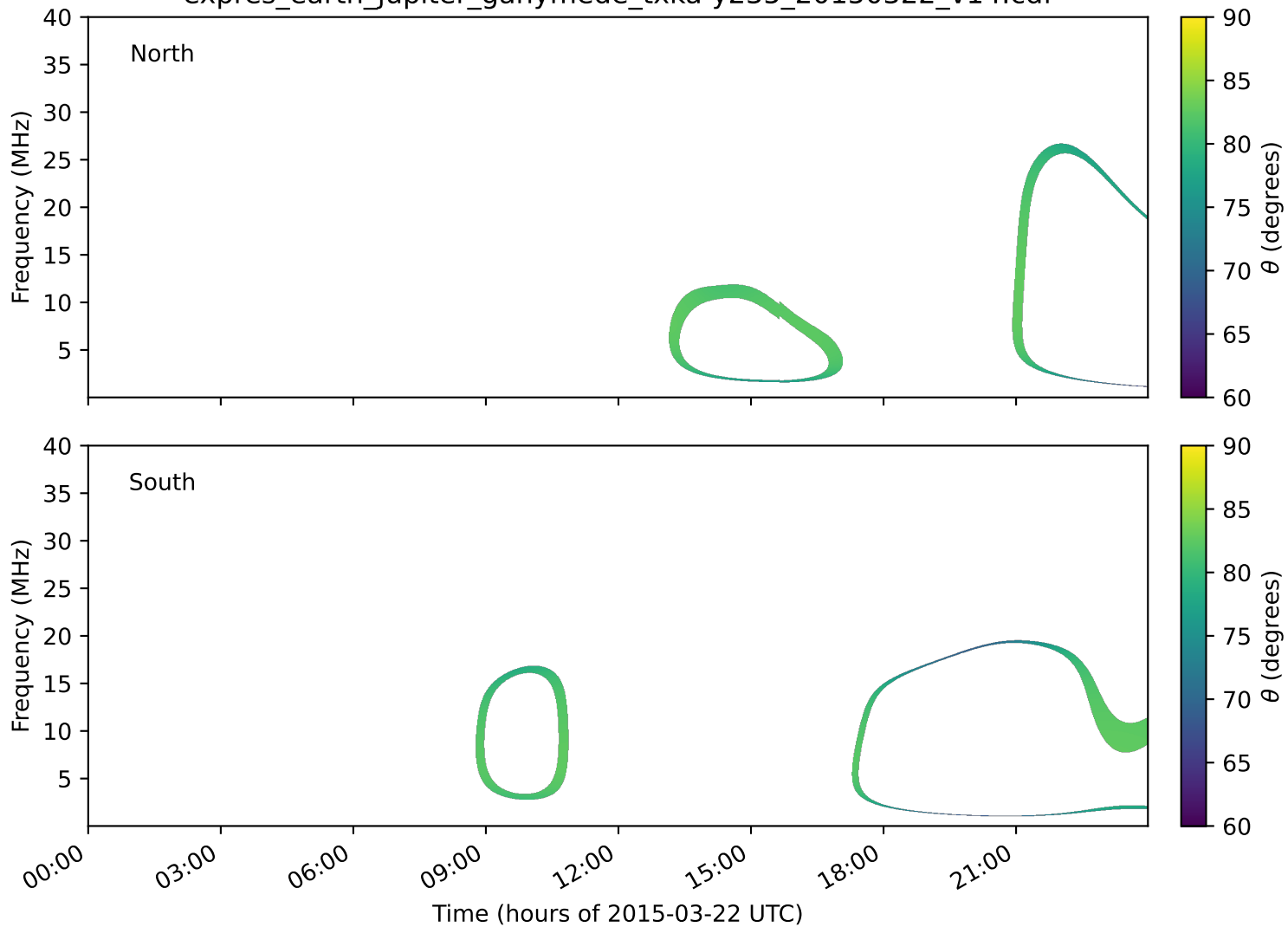
expres_earth_jupiter_ganymede_txka-y235_20150322_v14.cdf
