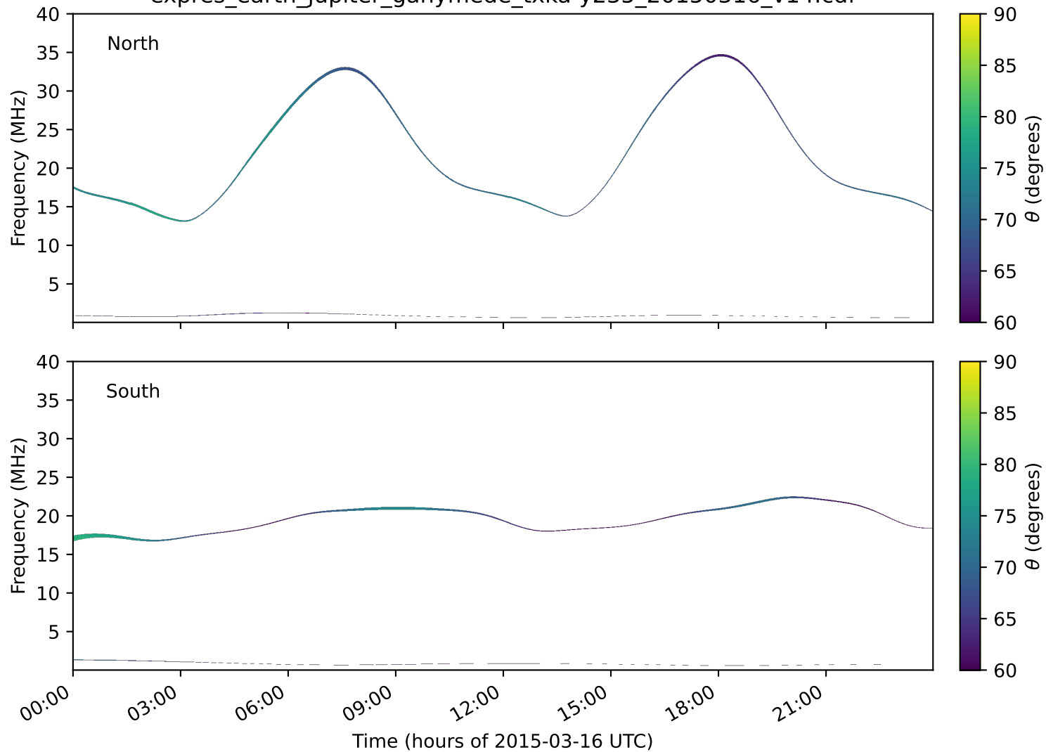
expres_earth_jupiter_ganymede_txka-y235_20150316_v14.cdf
