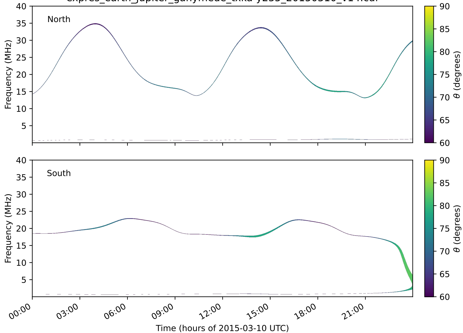
expres_earth_jupiter_ganymede_txka-y235_20150310_v14.cdf
