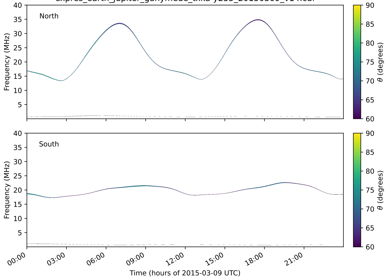
expres_earth_jupiter_ganymede_txka-y235_20150309_v14.cdf
