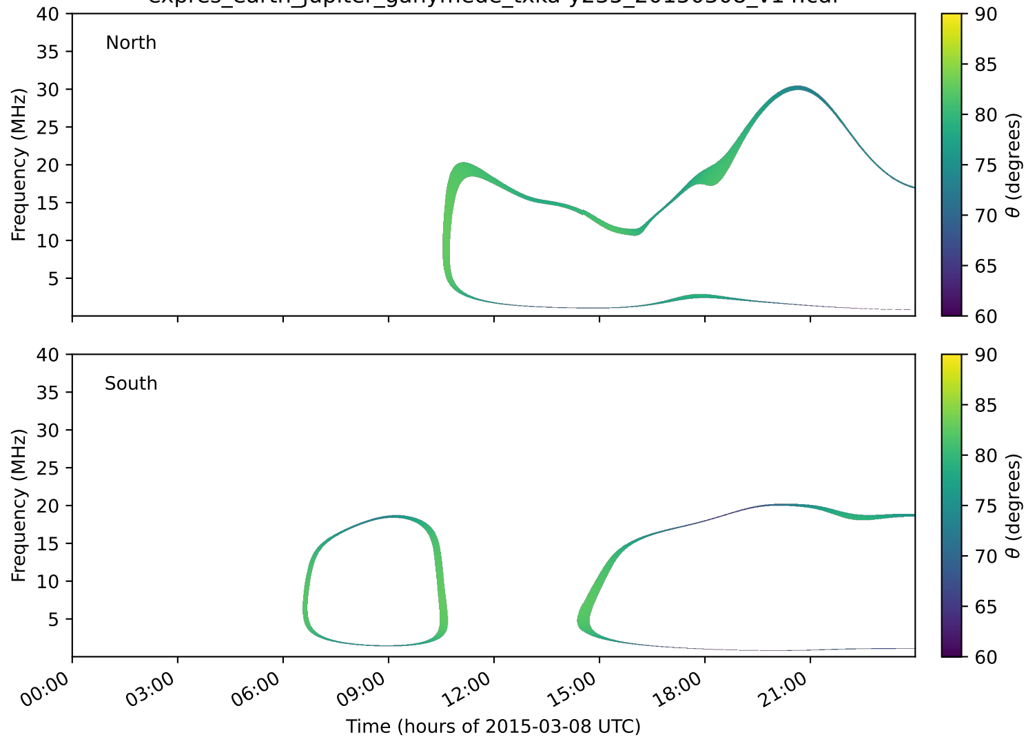
expres_earth_jupiter_ganymede_txka-y235_20150308_v14.cdf
