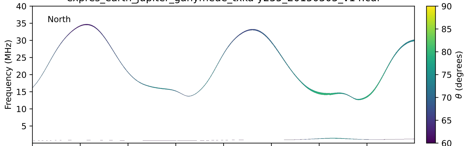
expres_earth_jupiter_ganymede_txka-y235_20150303_v14.cdf
