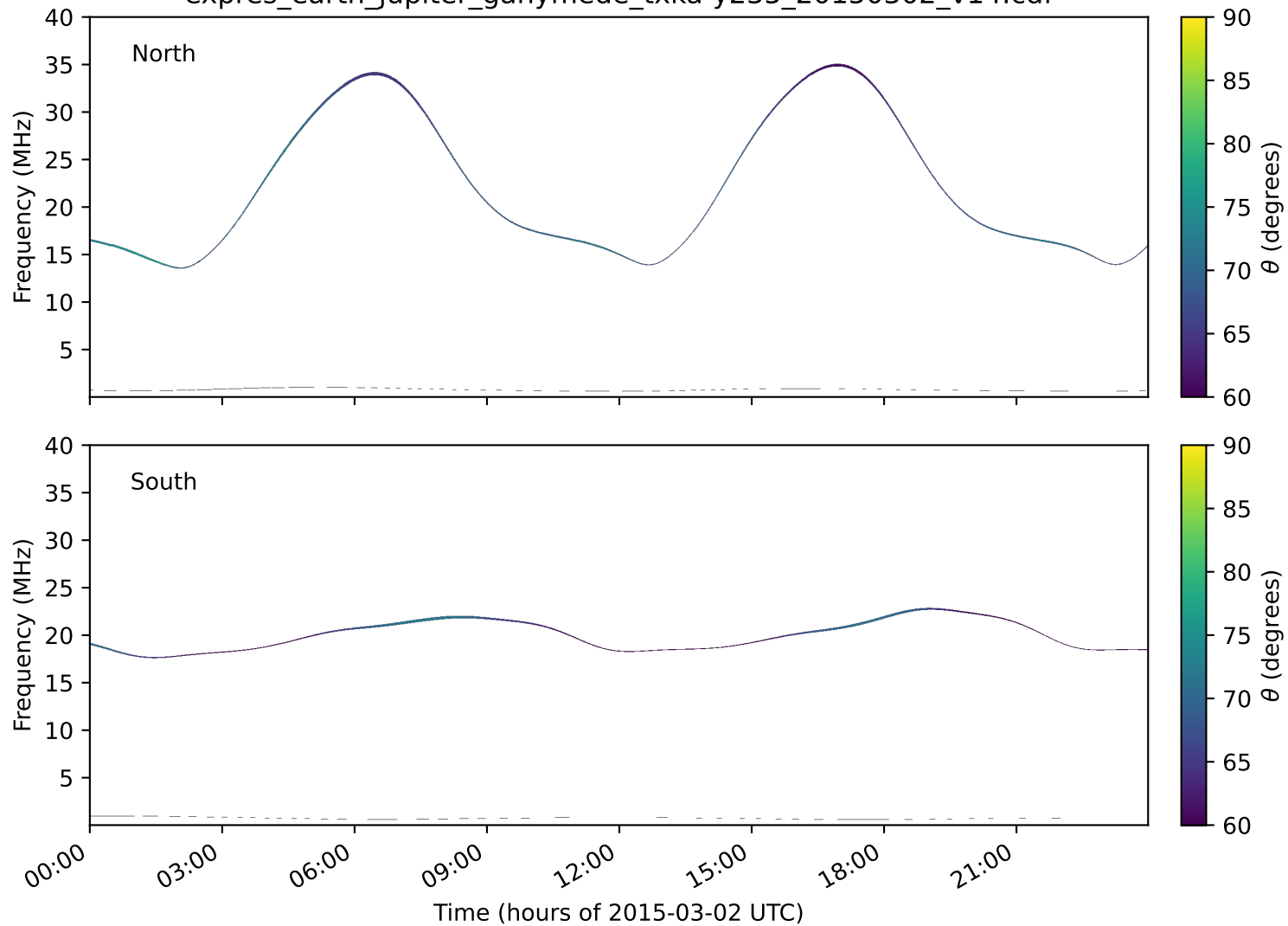
expres_earth_jupiter_ganymede_txka-y235_20150302_v14.cdf
