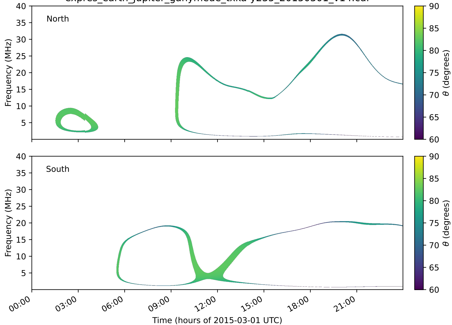
expres_earth_jupiter_ganymede_txka-y235_20150301_v14.cdf
