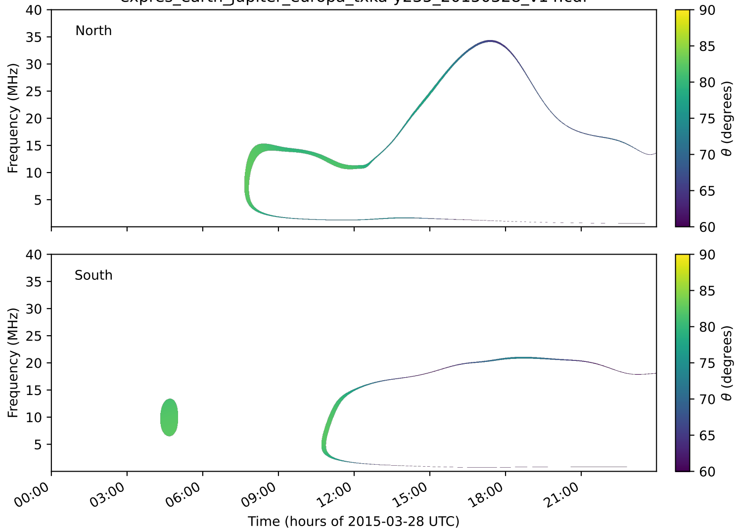
expres_earth_jupiter_europa_txka-y235_20150328_v14.cdf
