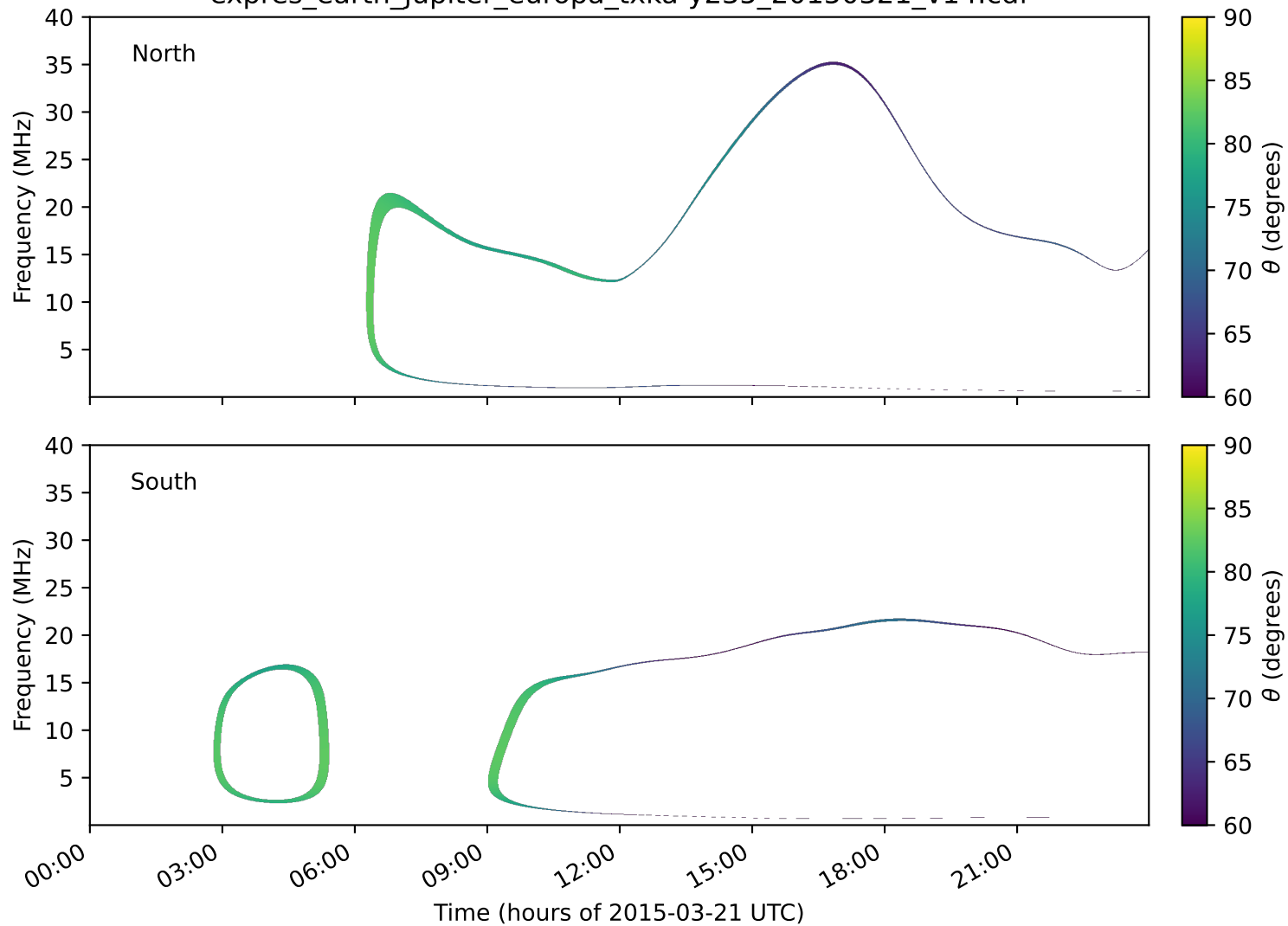
expres_earth_jupiter_europa_txka-y235_20150321_v14.cdf
