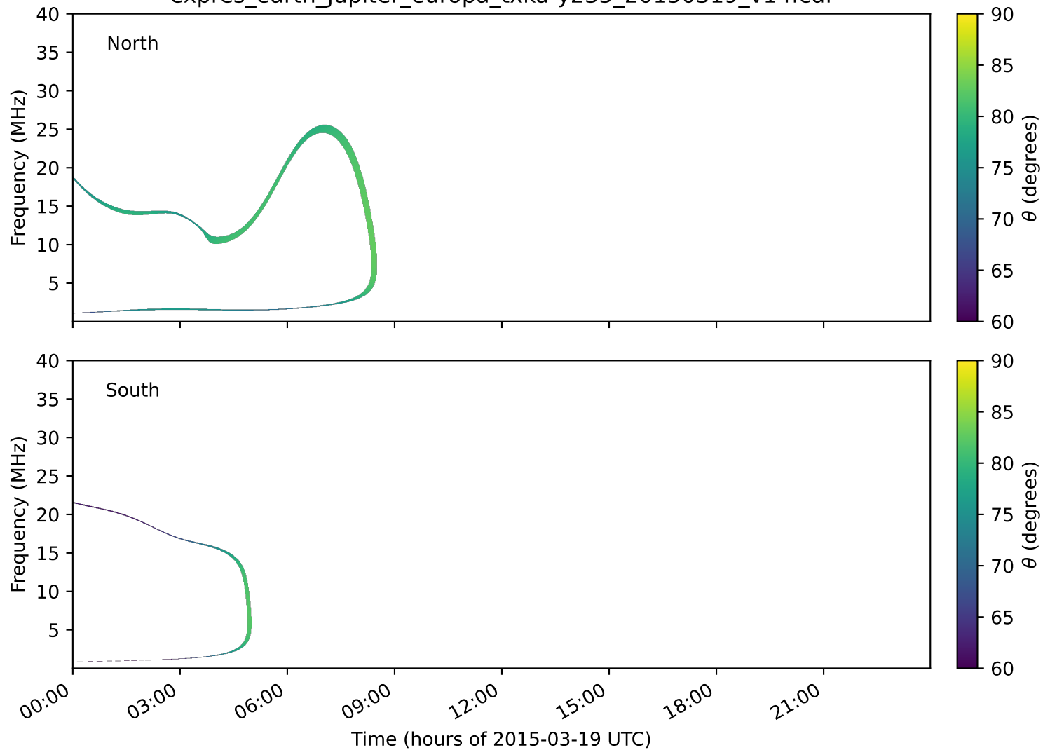
expres_earth_jupiter_europa_txka-y235_20150319_v14.cdf
