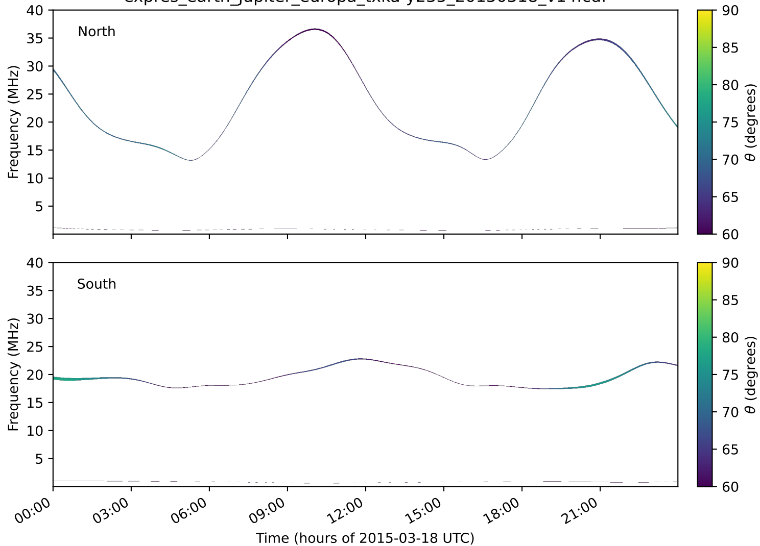
expres_earth_jupiter_europa_txka-y235_20150318_v14.cdf
