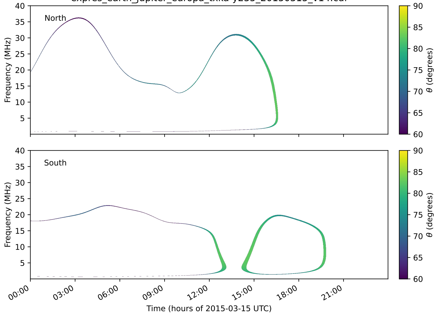
expres_earth_jupiter_europa_txka-y235_20150315_v14.cdf
