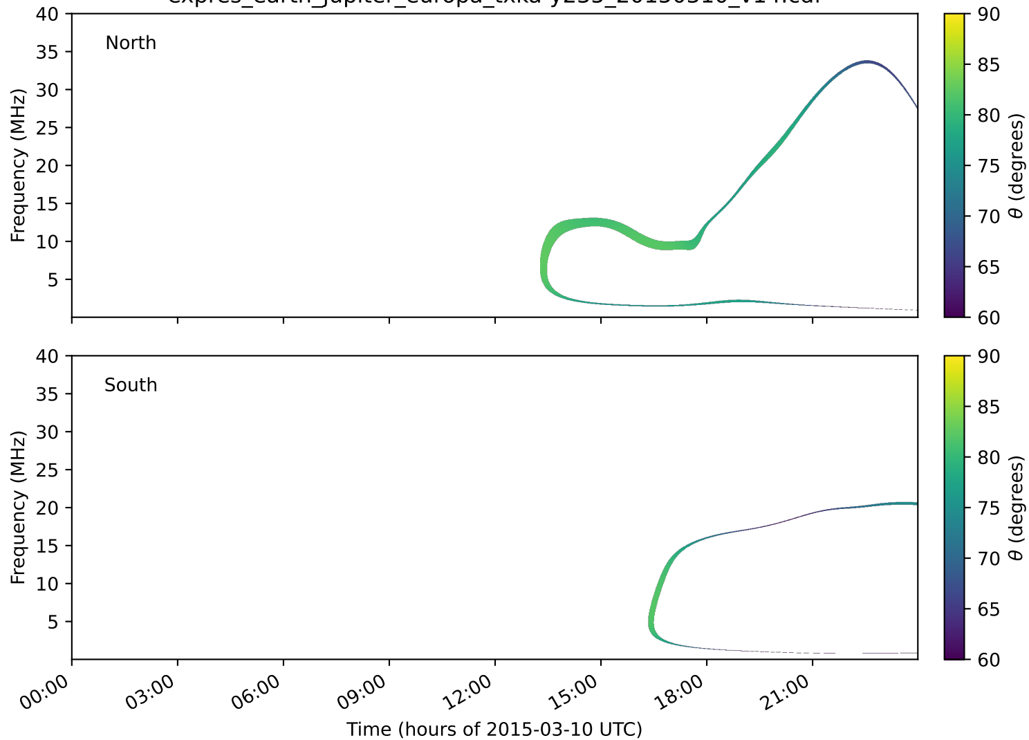
expres_earth_jupiter_europa_txka-y235_20150310_v14.cdf
